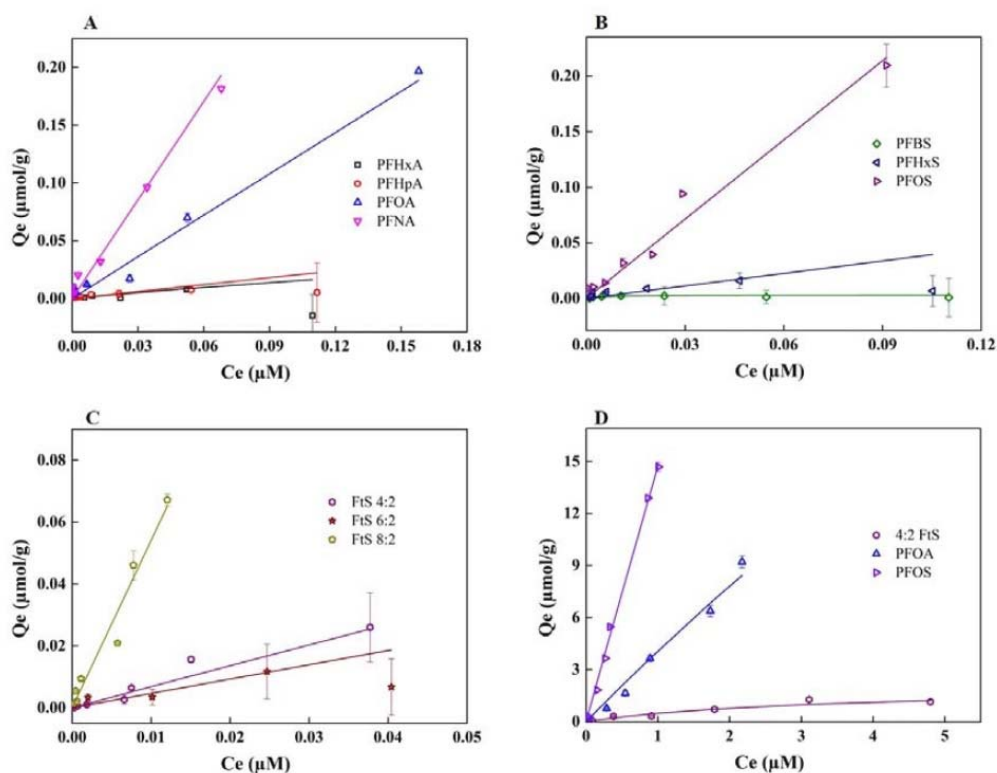
Figure 1 - (A, B, C) Langmuir sorption isotherm of the ten PFASs on the flocs ( C_0 = 0.001 - 0.1 \mu\text{M} , current density = 0.3 \text{ mA/cm}^2 , 20 \text{ mM Na}_2\text{SO}_4 , EC time = 120 min); (D) Langmuir sorption isotherm of single 4:2 FtS, PFOA and PFOS on the flocs, respectively. ( C_0 = 0.002 - 5 \mu\text{M} , current density = 0.3 \text{ mA/cm}^2 , 20 \text{ mM Na}_2\text{SO}_4 , EC time = 120 min).
